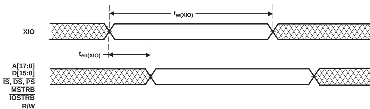
Figure 5-14. XIO Timing
