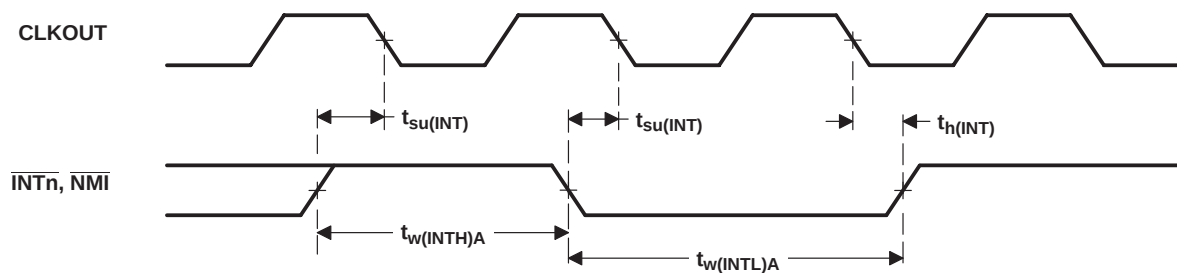
Figure 5-13. Interrupt Timing
